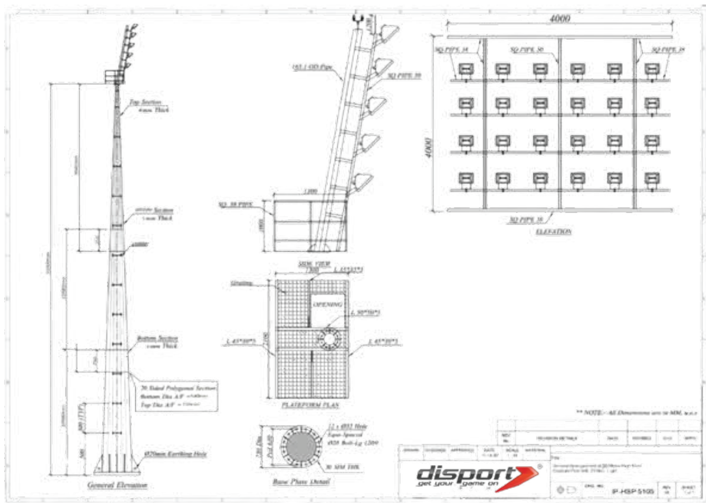
STADIUM MAST POLE PICTURE DRAWING
